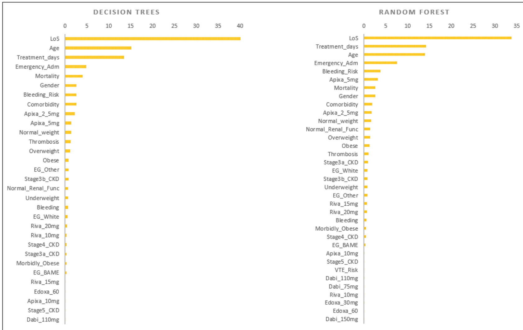
Figure S2: Ranking of features with the overall patient dataset according to their importance in contributing to stroke using Random Forest and Decision Trees. EG=ethnic group
