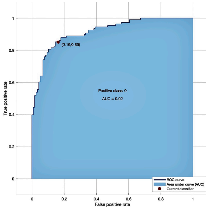
Fig. 6. ROC curve of Logistic regression for first dataset.
