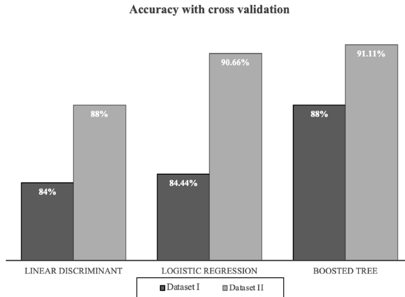
Fig. 10. Classification accuracy for Machine learning techniques for both datasets with Five-fold cross validation.
