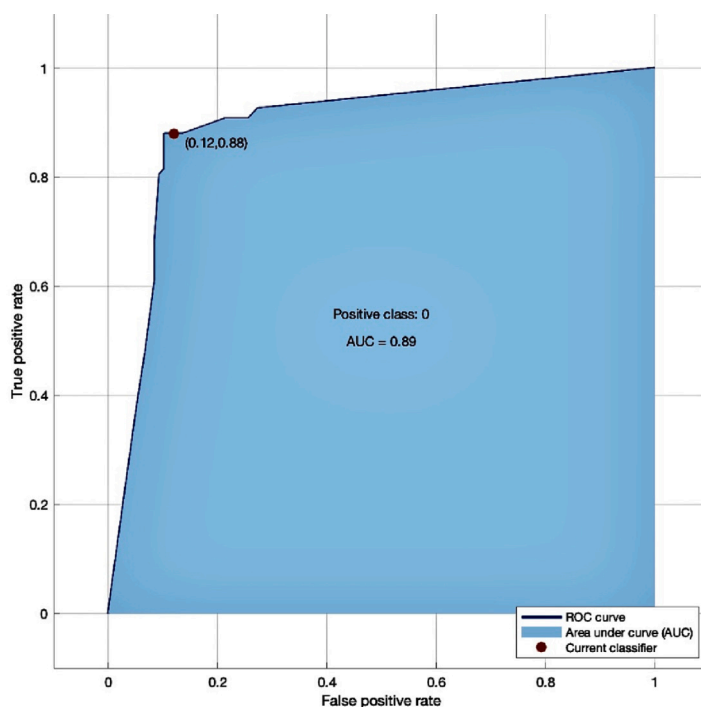
Fig. 4. ROC curve of Boosted Trees for the first dataset.
