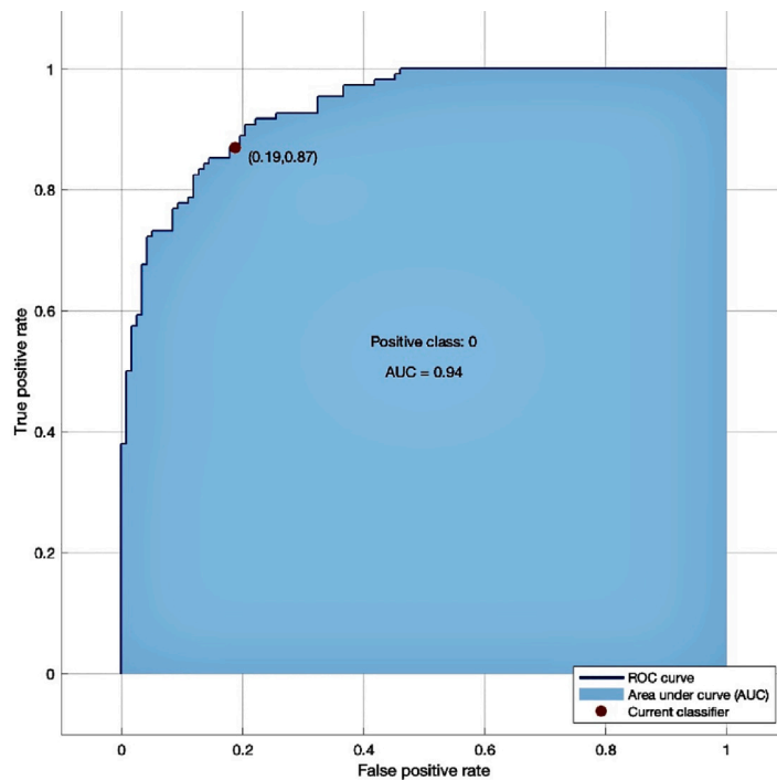
Fig. 5. The ROC curve depicting the performance of Linear Discriminant for the first dataset.
