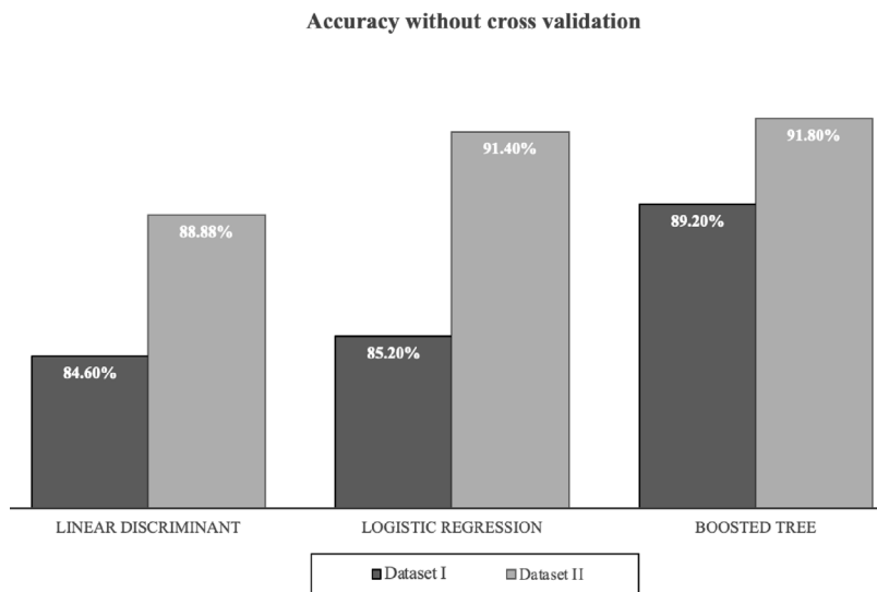
Fig. 11. Classification accuracy for Machine learning techniques for both datasets without validation.
