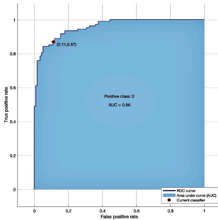
Fig. 8. ROC curve of Linear Discriminant for the second dataset.
