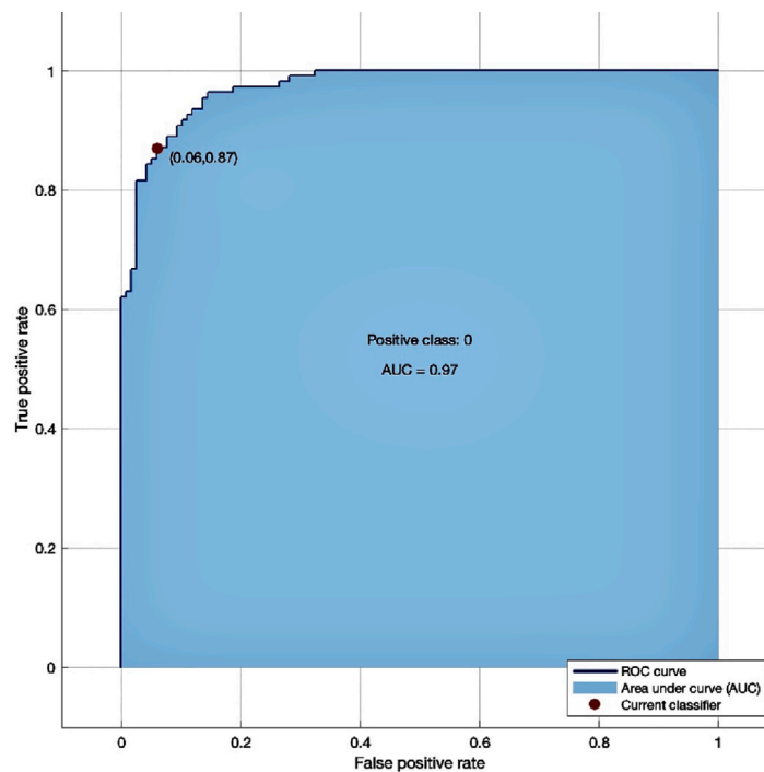
Fig. 9. ROC curve of Logistic regression for the second dataset.
