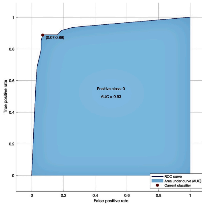
Fig. 7. ROC curve of Boosted Trees for second data-set.
