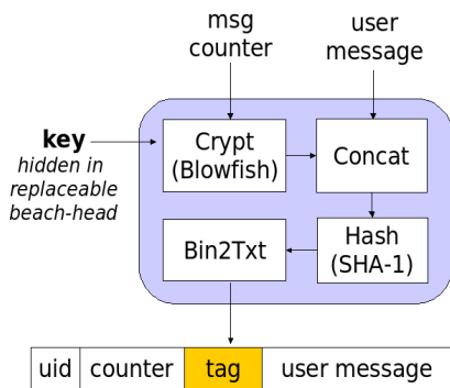
Figure 3: Tag generation schema
