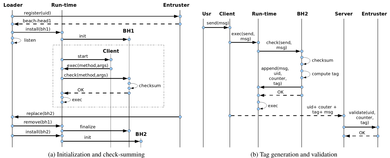
Figure 2: Sequence diagram
