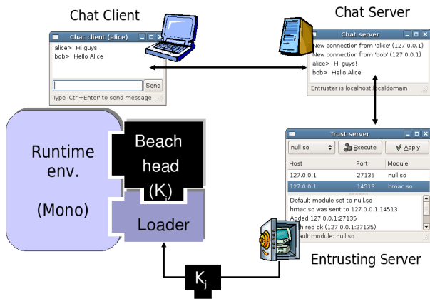
Figure 1: Prototype architecture
