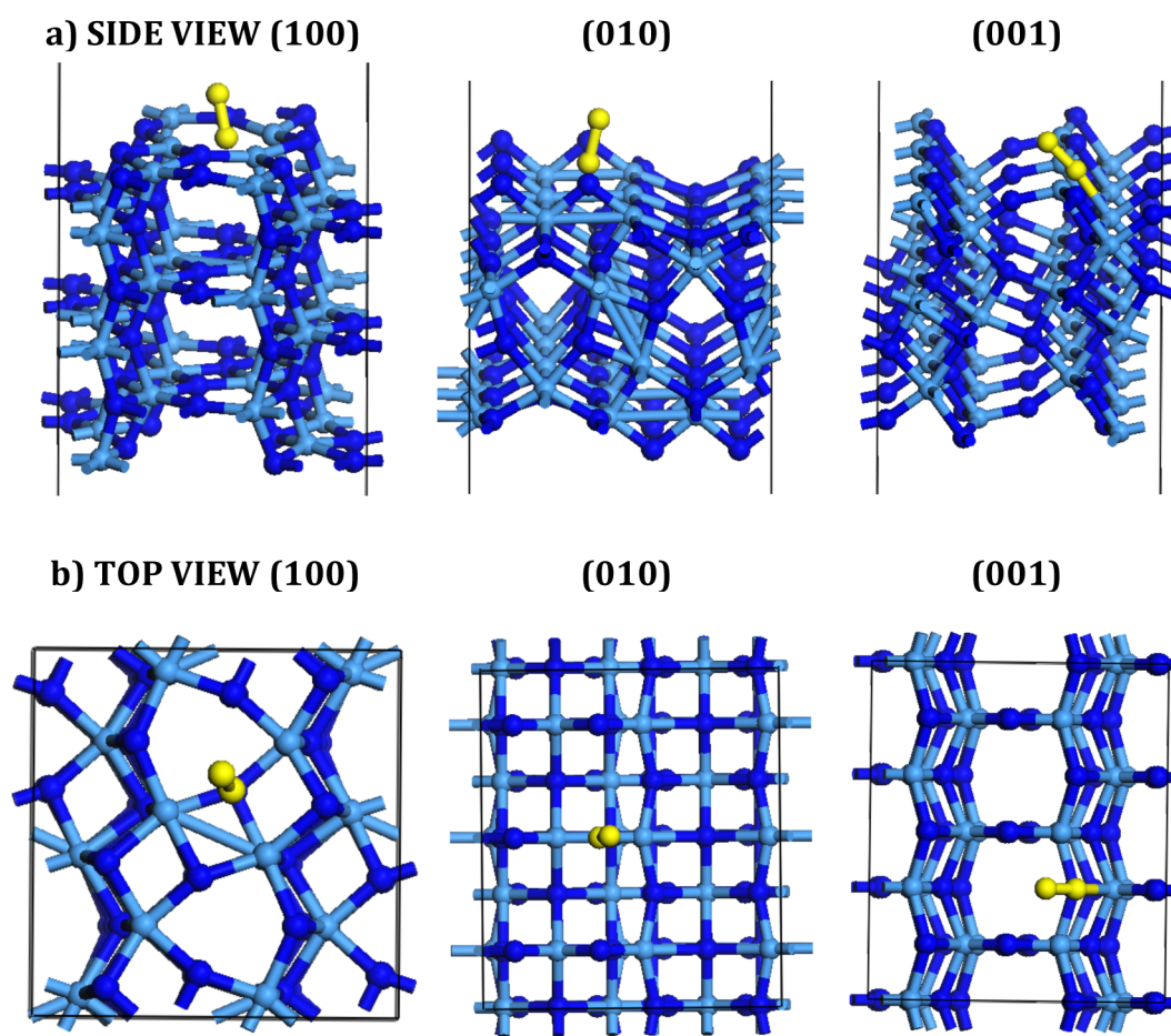
Fig. 1 (a) Side view and b) top view of \text{Ta}_3\text{N}_5 showing in yellow dinitrogen initial structure at the nitrogen vacancy of the corresponding surface (100), (010) and (001), respectively.
