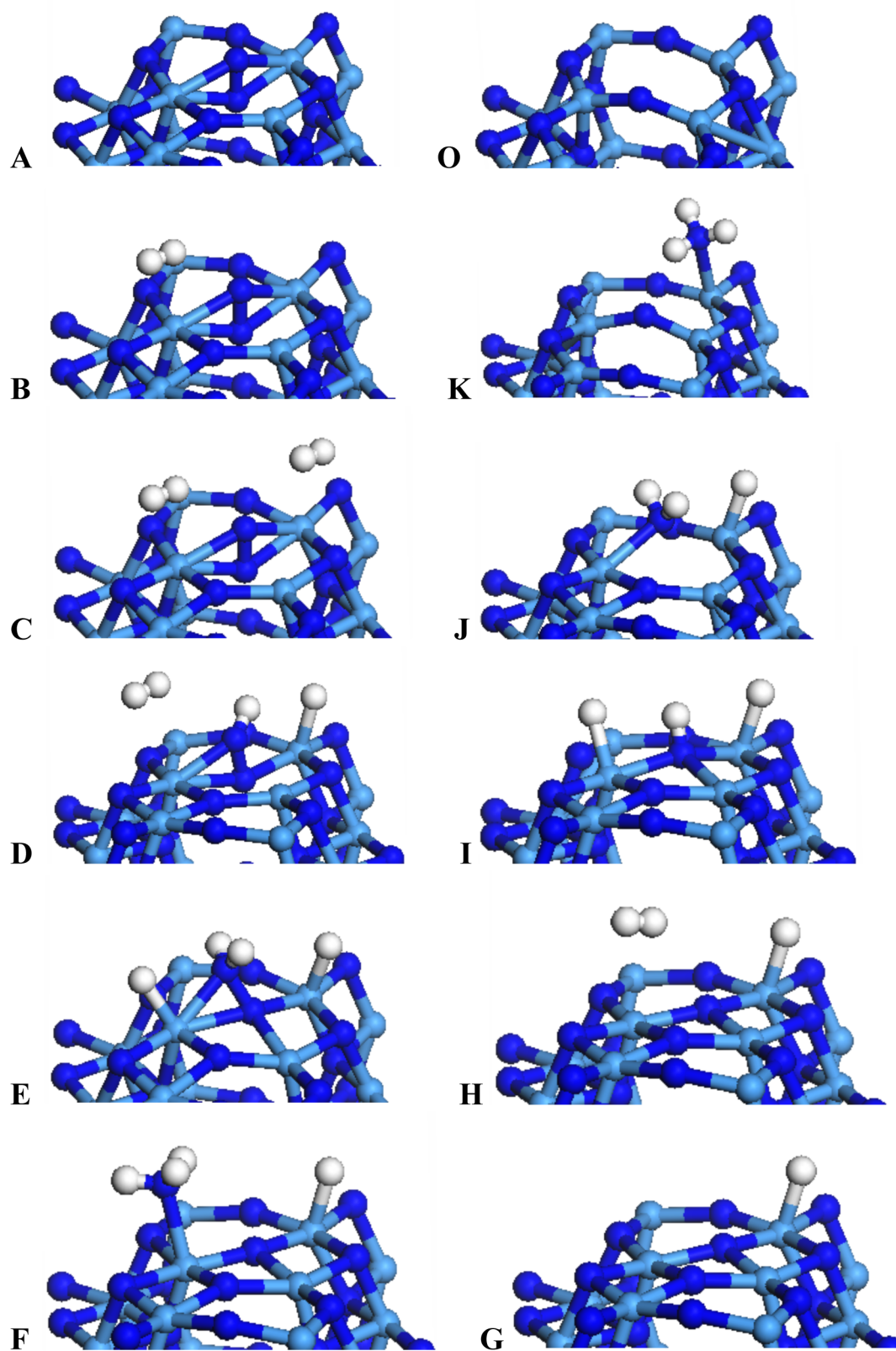
Fig. 3 Ball and stick model of the mechanism of ammonia synthesis at nitrogen vacancies of the \text{Ta}_3\text{N}_5 -(100) surface. The mechanism initiates at O with the adsorption of dinitrogen to a nitrogen vacancy.
