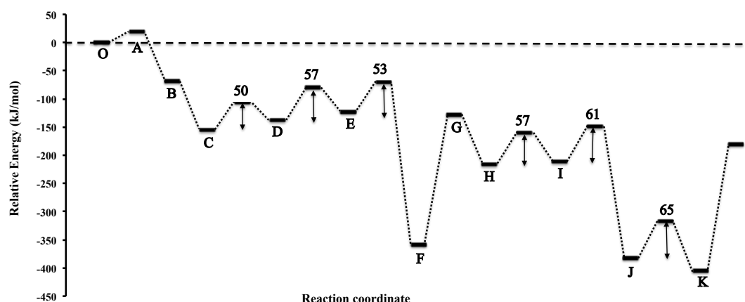
Fig. 4 Potential energy diagram of ammonia synthesis reaction mechanism on (100)- \text{Ta}_3\text{N}_5 surfaces in the presence of nitrogen vacancies.
