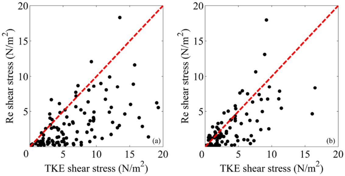
Figure 3. Comparison of the one-second mean Reynolds and TKE shear stresses from (a) above the measured mean critical velocity ( \bar{u} > \bar{u}_{cr, measured} ) and (b) below the measured mean critical velocity ( \bar{u} < \bar{u}_{cr, measured} ) experiments with a two-minute period. The dashed red line defines the equality.
