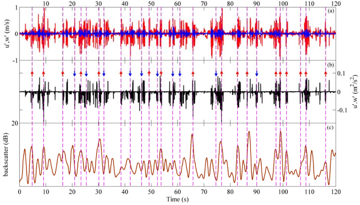
Figure 4. Time series records from the above measured mean critical velocity experiment ( \bar{u} > \bar{u}_{cr, measured} ): (a) turbulent velocity ( u' - red in color, w' - blue in color); (b) turbulent Reynolds shear stress ( u'w' ), showing the ejection (red up arrows) and sweep (blue down arrows) events; (c) one-second mean of the backscatter.
