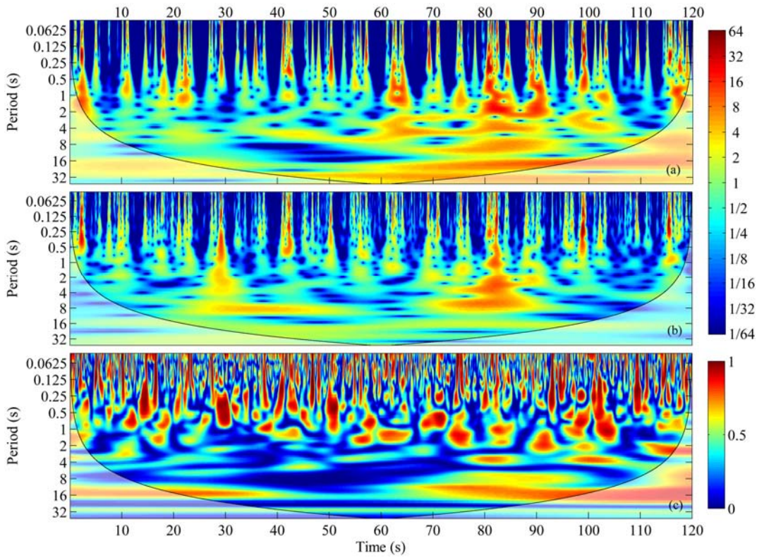
Figure 10. Wavelet power spectra (Morlet wavelet) for below the measured mean critical velocity experiment ( \bar{u} < \bar{u}_{cr, \text{measured}} ) for a two-minute period showing the (a) momentum flux ( u'w' ), (b) sediment flux ( c'w' ), and (c) coherence between the momentum and sediment fluxes.
