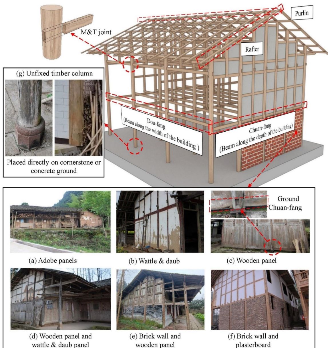
Fig. 6: The construction form and common wall types of Chuan-dou timber structures (Liang et al. 2022)
