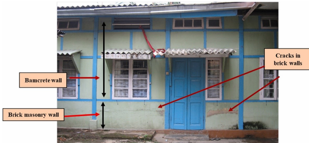
(a) Exterior view
