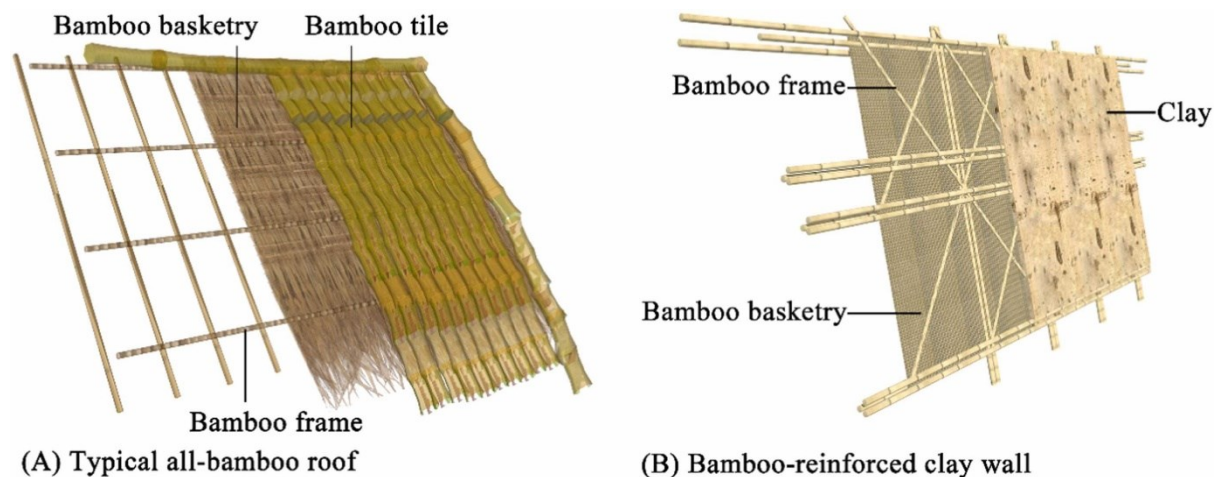
Fig. 5: Traditional bamboo-bearing structures (Ding & Xian, 2024)
