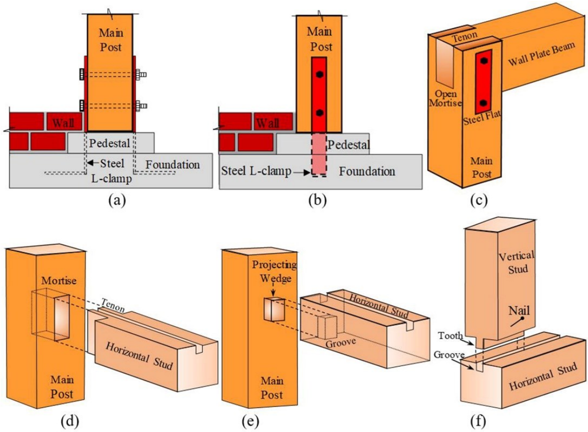
Fig. 3: Details of joints used in typical Assam-type houses: (a) Joint A, (b) Joint B, (c) Joint C, (d) Joint D, (e) Joint E, and (f) Joint F (Chand et al. 2020b).
