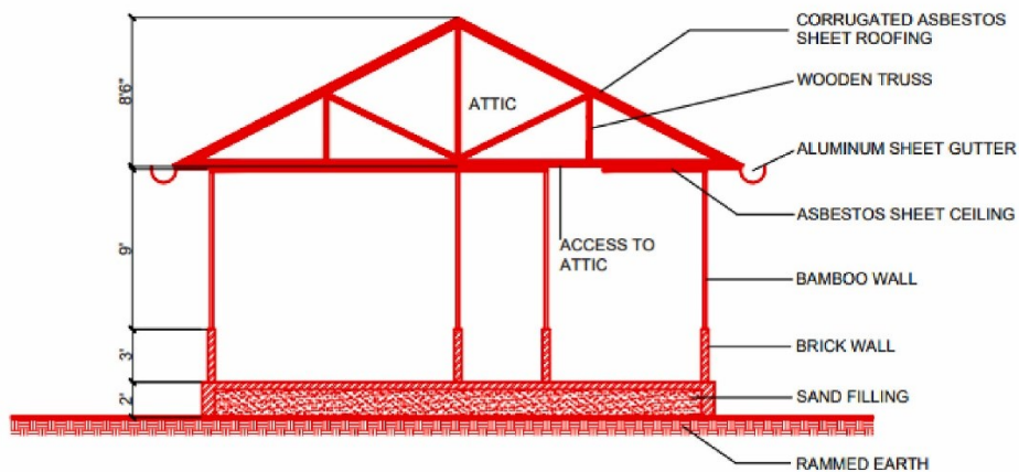
(b) Section
