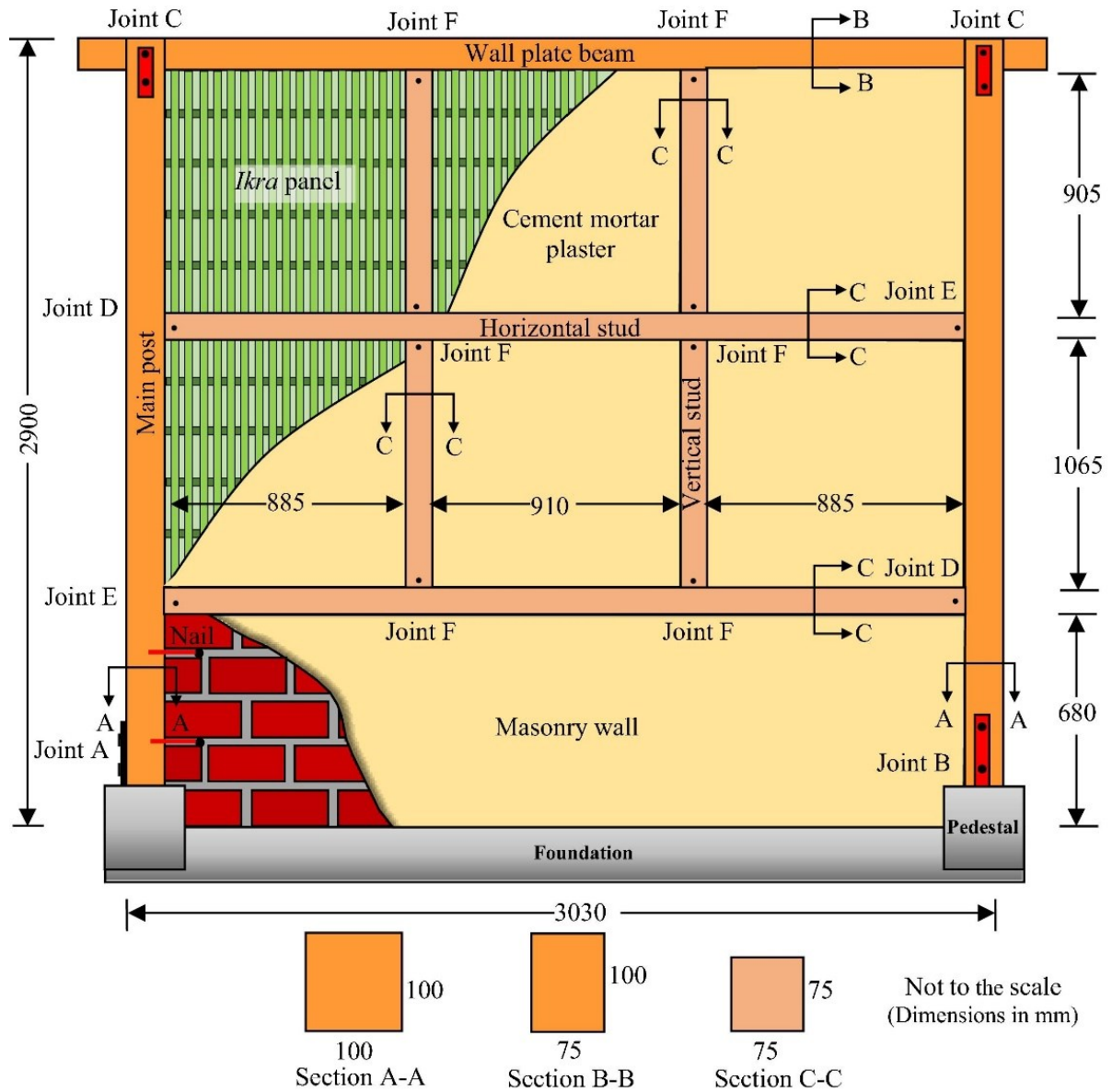
Fig. 2: Details of a typical frame of Assam-type house (Chand et al. 2020b).
