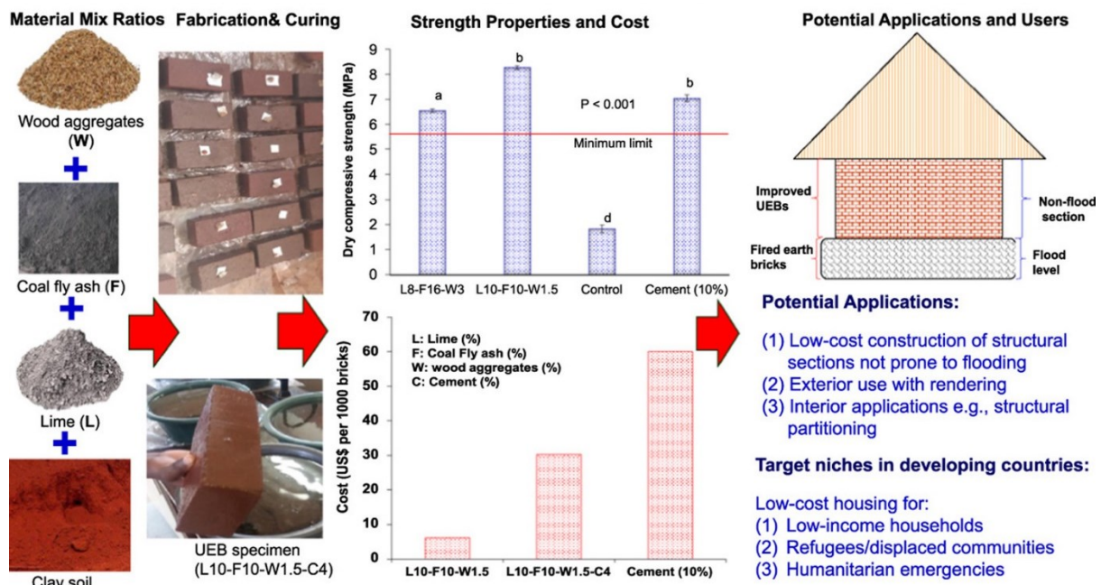
Fig. 10: Development, Evaluation and Potential Application of Improved Unfired Earth Bricks (Masuka et al. 2018)
