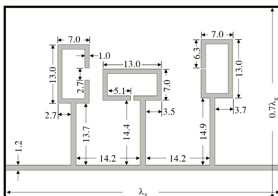
Figure 10. Microstrip bandstop filter layout with dimension. All dimensions are in millimetre, reproduced courtesy of The Electromagnetics Academy
