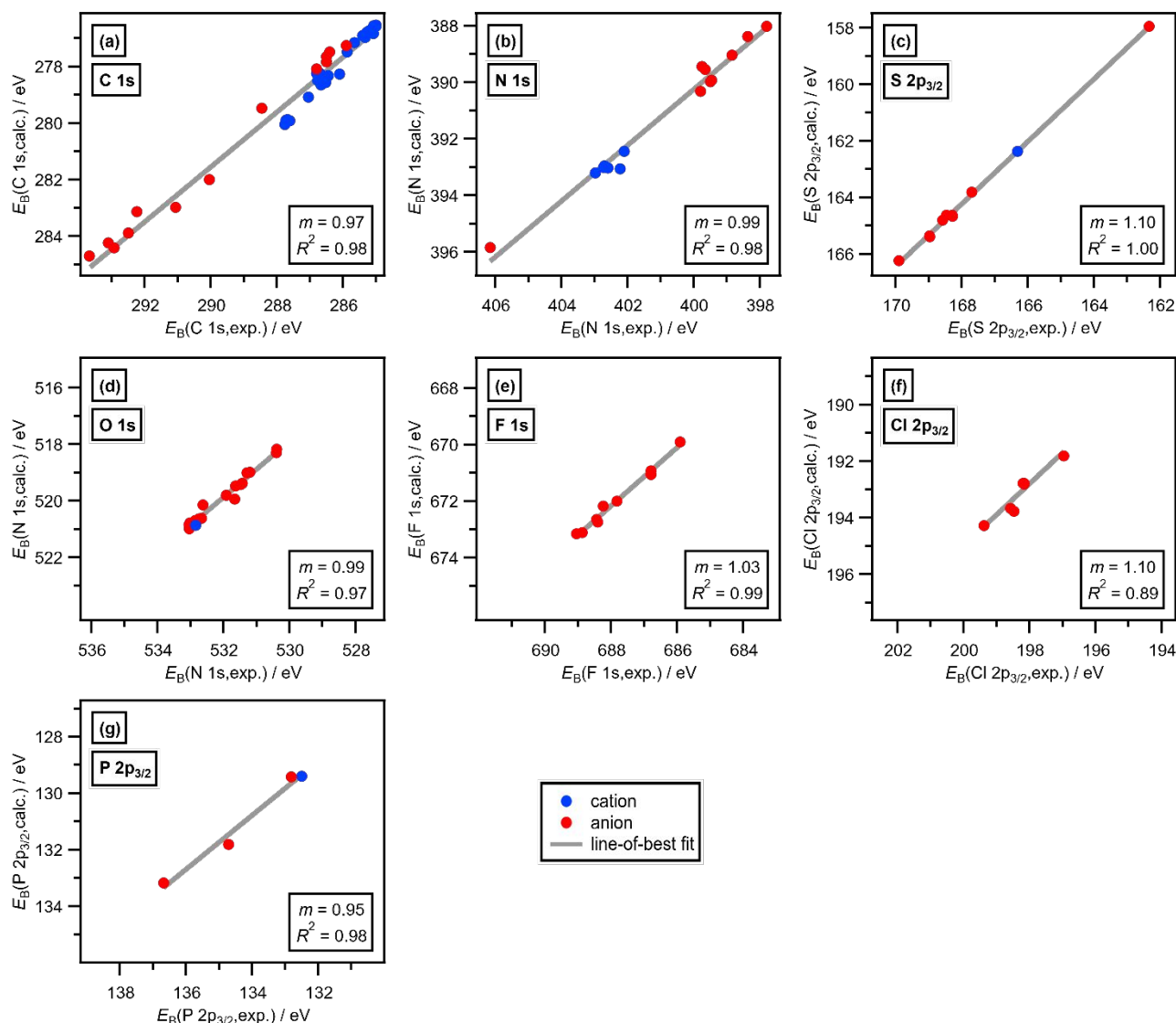
Figure 1. Calculated binding energy, E_B(\text{calc.}) from lone-ion-SMD against experimental XPS binding energy, E_B(\text{exp.}) for: (a) C 1s, (b) N 1s, (c) S 2p_{3/2} , (d) O 1s, (e) F 1s, (f) Cl 2p_{3/2} , (g) P 2p_{3/2} . m is the gradient of each line-of-best fit. The experimental uncertainty is \pm 0.10 eV; the calculated uncertainty is \pm 0.20 eV.
