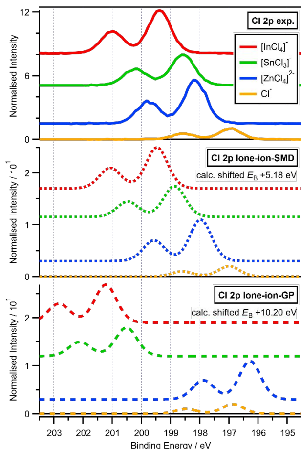
Figure 2. Experimental and calculated Cl 2p XPS for [\text{C}_8\text{C}_1\text{Im}][\text{A}] where \text{A} = \text{Cl}^- , [\text{ZnCl}_4]^{2-} , [\text{SnCl}_3]^- and [\text{InCl}_4]^- : (top) experimental Cl 2p XPS (vertically offset for clarity); (middle) calculated Cl 2p XPS for lone-ion-SMD of the anions ( E_B (correction) = +5.18 eV, vertically offset for clarity); (bottom) calculated Cl 2p XPS for lone-ion-gas-phase (GP) of the anions ( E_B (correction) = +10.20 eV, vertically offset for clarity). Experimental XP spectra are area normalised and charge referenced using methods given in ESI Section 5.
