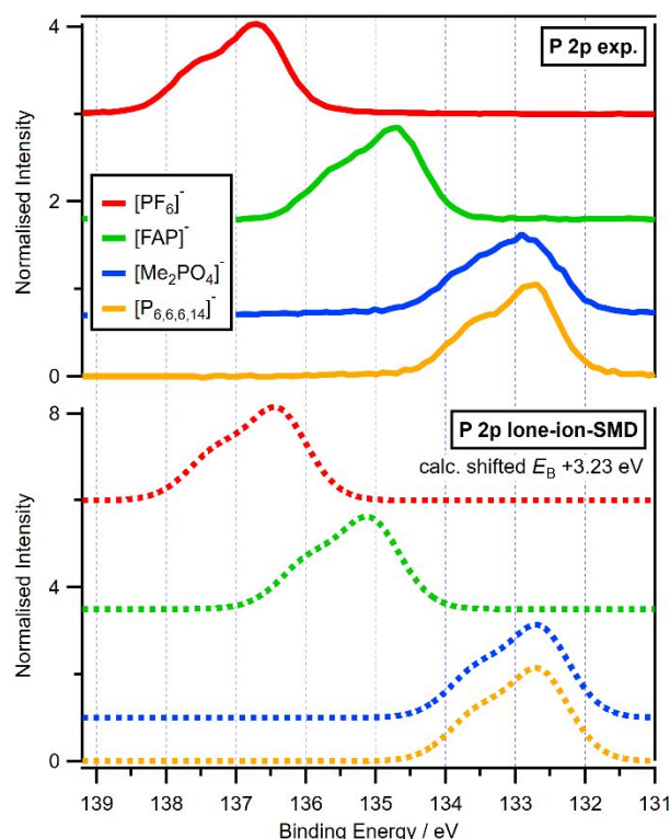
Figure 4. Experimental and calculated P 2p XPS for four P-containing ILs and four lone P-containing lone ions: (top) experimental P 2p XPS for [C_4C_1Im][PF_6] , [C_2C_1Im][FAP] , [C_4C_1Im][Me_2PO_4] and [P_{6,6,6,14}][NTf_2] (vertically offset for clarity); (bottom) calculated P 2p XPS for lone-ion-SMD of the ions [PF_6]^- , [FAP]^- , [Me_2PO_4]^- and [P_{6,6,6,14}]^+ ( E_B(\text{correction}) = +3.23 eV, vertically offset for clarity). Experimental XP spectra are area normalised and charge referenced using methods given in ESI Section 5.
