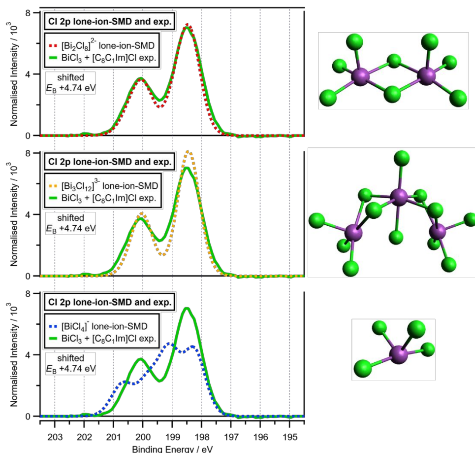
Figure 5. Experimental Cl 2p XPS for x = 0.5 \text{ BiCl}_3 dissolved in [\text{C}_8\text{C}_1\text{Im}]\text{Cl} (top, middle and bottom) and calculated Cl 2p XPS for lone-ion-SMD of the anions ( E_B(\text{correction}) = +4.74 \text{ eV} ): (top) [\text{Bi}_2\text{Cl}_8]^{2-} ; (middle) [\text{Bi}_3\text{Cl}_{12}]^{3-} ; (bottom) [\text{BiCl}_4]^- . The experimental XP spectrum is charge referenced using methods given in ESI Section 5. The structures are given on the right-hand side.
