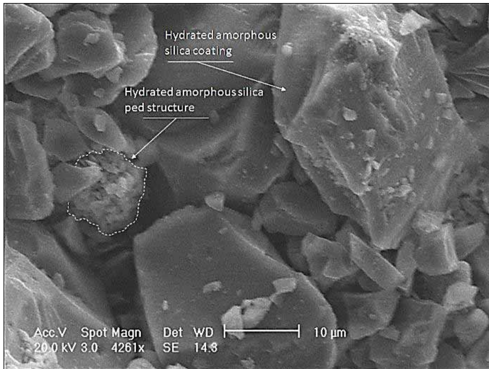
Fig. 1 Horizontal alignment, silica-indurate silt in hot environment
