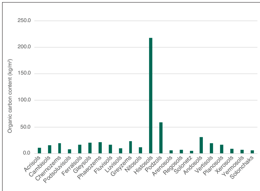
2 Organic carbon content for FAO-UNESCO soil units to 2 m depth
