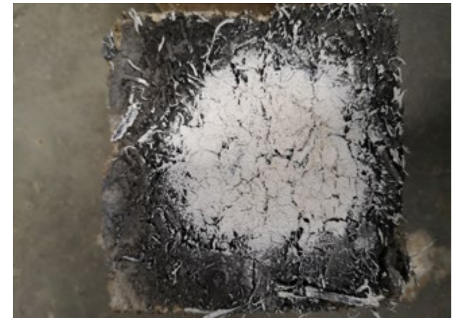
Fig.12 - Prototype 4
