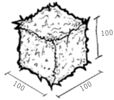
SUGARCRETE BRICK
