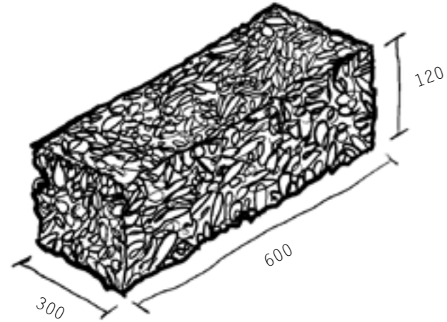
HEMP BRICK
