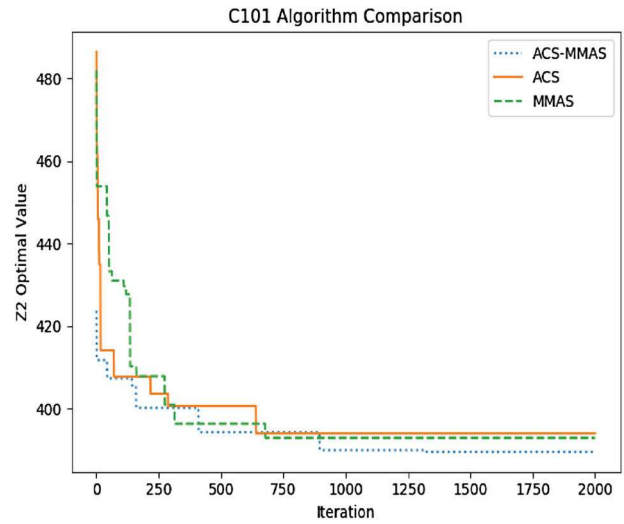
(b) Comparison of algorithm convergence in C101 example
