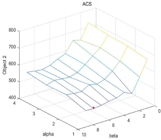
(a) ACS algorithm and parameter
