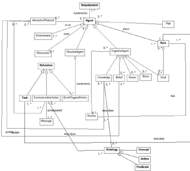
Fig. 18. Final metamodel for the agent perspective proposed by Azaiez et al. (from [8]).
