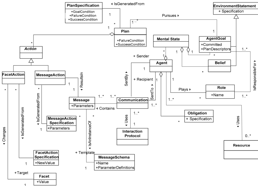
Fig. 15. Runtime agent-internal classes.
