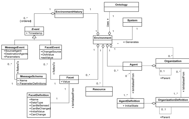
Fig. 14. Runtime agent-external classes.
