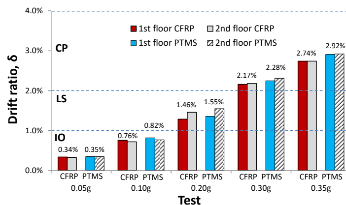
Fig. 11 - Interstorey drift ratio of 1 st and 2 nd floors during phase 4 (Y direction)
