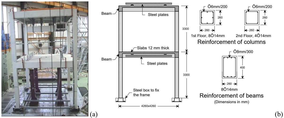
Fig. 1 - ECOLADER frame building: (a) general view, (b) geometry of the frame and structural elements
