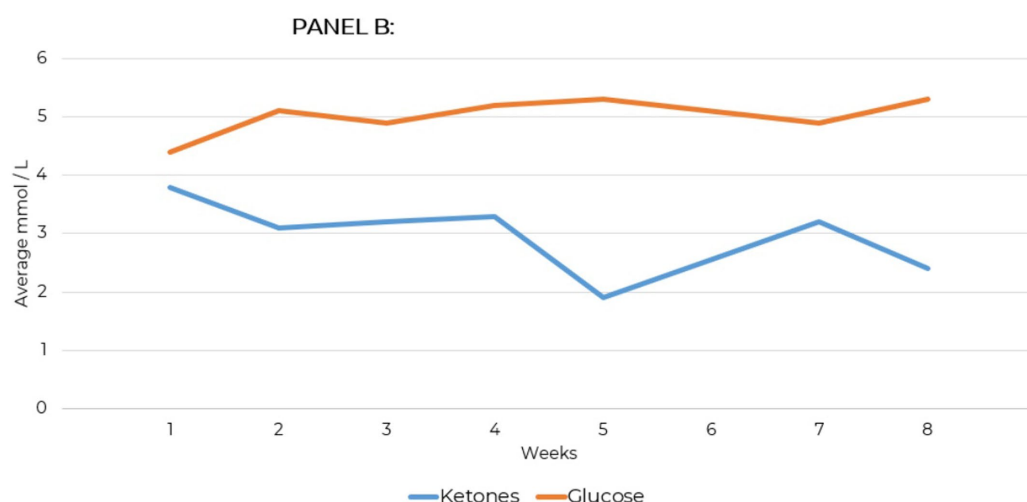
FIGURE 1 Weekly average ketone and measures for case presentations 1 and 2. (A) Average glucose/ketone levels. (B) Average glucose/ketone levels.
