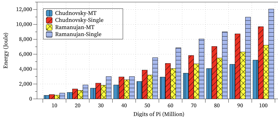
Figure 5: Energy consumption of Pi algorithms
