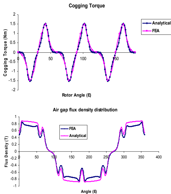
Figure 4. Comparison of Finite Element and analytical results for taper with M_{off} = 3.35\text{mm}
