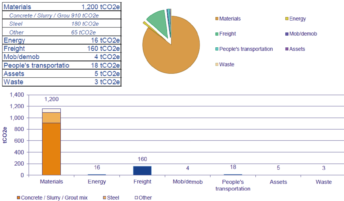
Fig. 9(a) Carbon footprint of benchmark problem for piled foundation adoption
