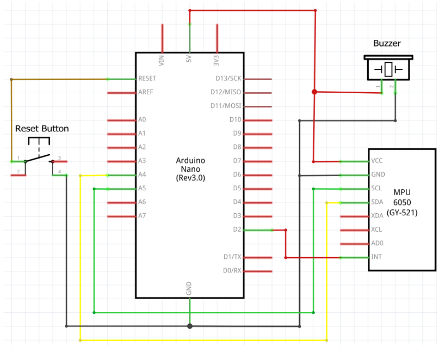
Figure 3: Schematic View
