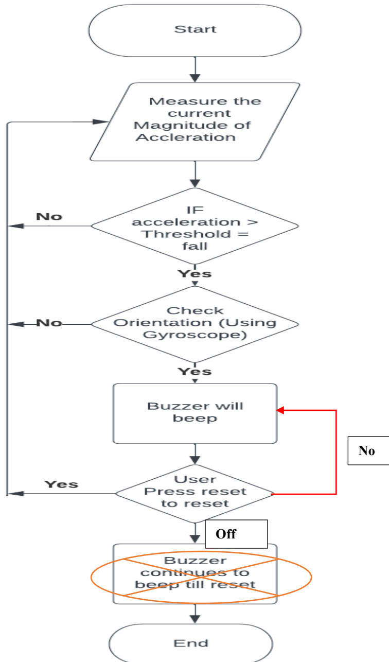
Figure 2: Threshold-Base Algorithm Design
