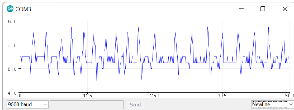
Figure 8: Acceleration Graph for Sitting and Standing (ADL 2)
