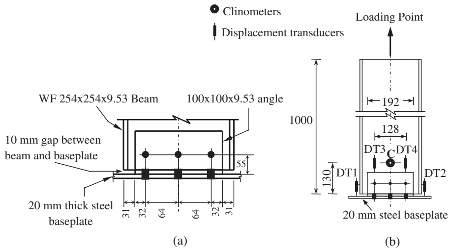
Fig. 2. Connection details and instrumentation for a 254 × 254 × 9.53 mm specimen (all dimensions are in mm): (a) connection details; (b) instrumentation.
