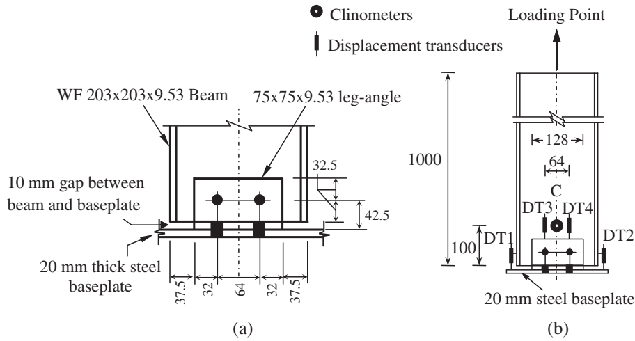
Fig. 3. Connection details and instrumentation for a 203 × 203 × 9.53 mm specimen (all dimensions are in mm): (a) connection details; (b) instrumentation.
