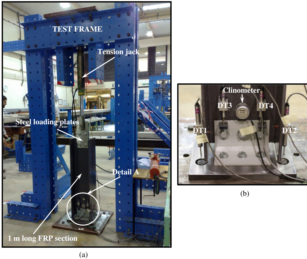
Fig. 1. General test arrangement for tension pull test with a 254 × 254 × 9.53 mm specimen: (a) test arrangement; (b) detail A.
