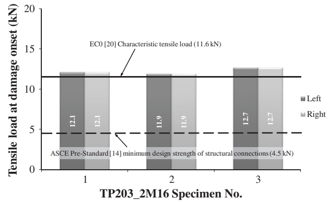
Fig. 9. Characteristic tensile loads for batch TP203_2M16.
