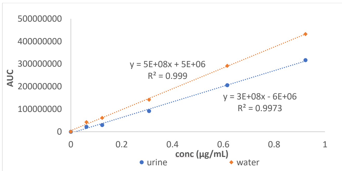
Figure S1. Matrix effect. Comparison of linearity of working solutions prepared from urine samples to linearity in deionised water. Representative results obtained for the compound 510.3994 m/z.
