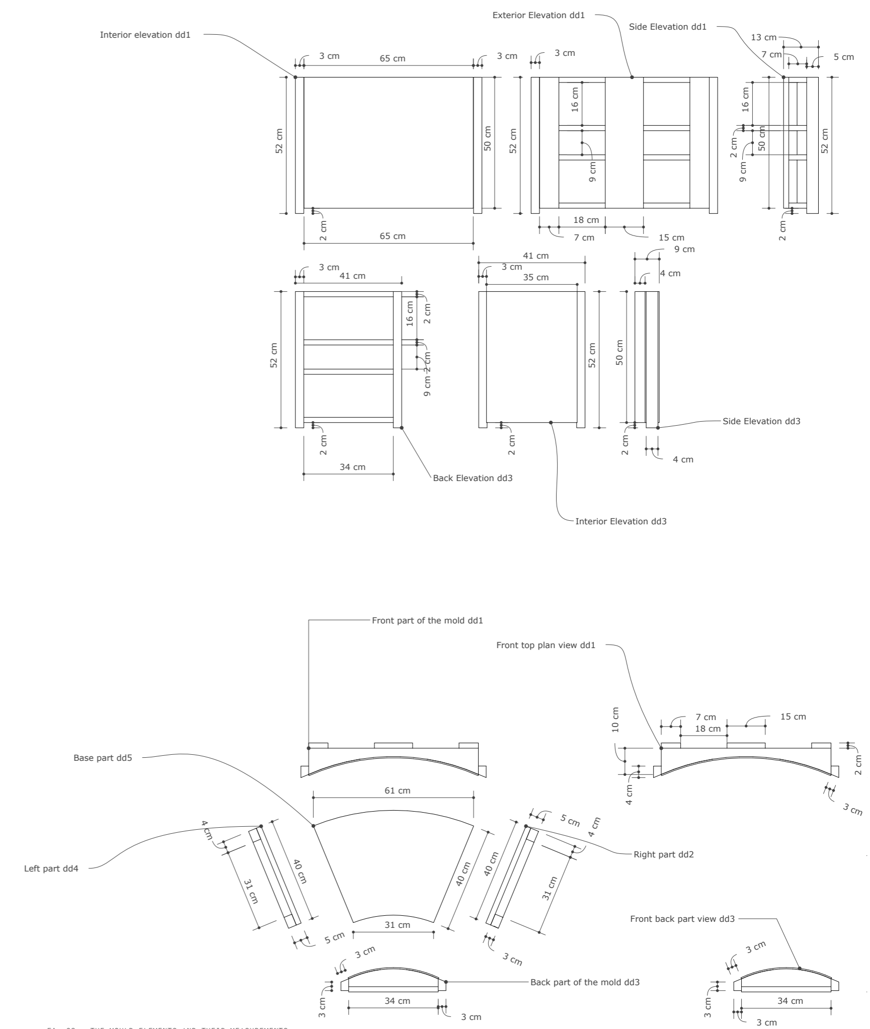
Fig.28 - THE MOULD ELEMENTS AND THEIR MEASUREMENTS
