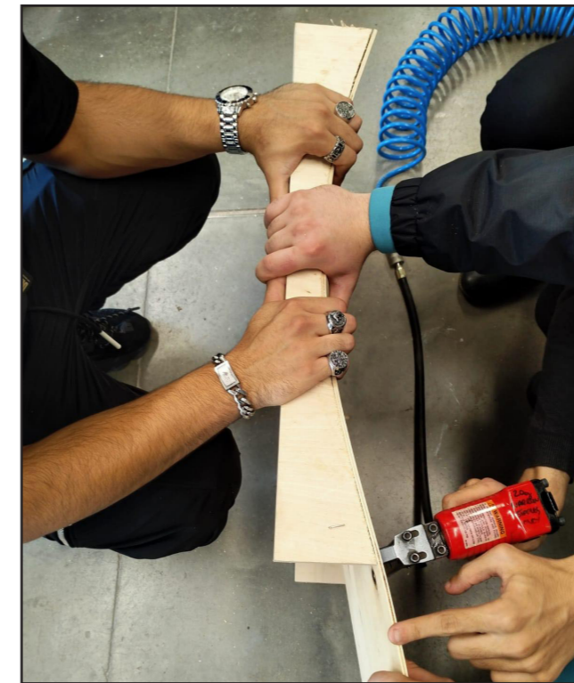
Fig. 53 - STAPLING THE TOP SIDE OF THE PLYWOOD SHEET
