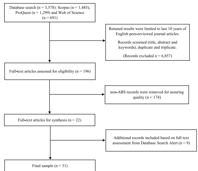
Fig. 1. PRISMA outline.
