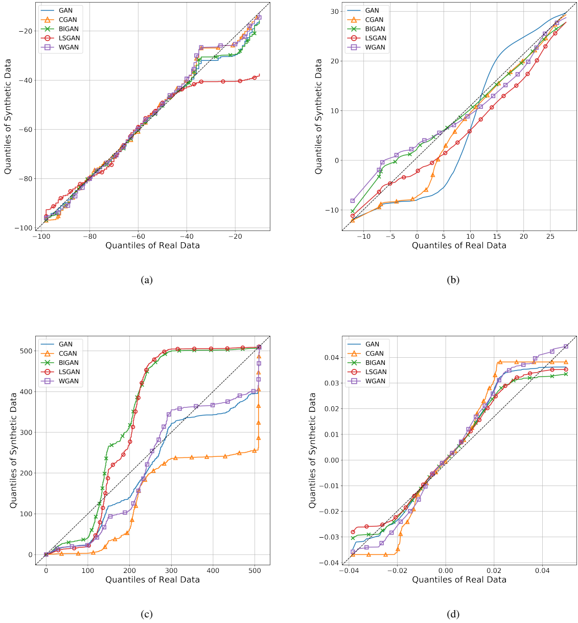
Figure 8: Q-Q plot for a) RSS dataset, b) CSI dataset, c) KDD99 dataset, column “count”, and d) RADIOML datasets.
