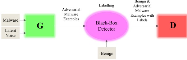
Figure 6: MalGAN architecture [122].
