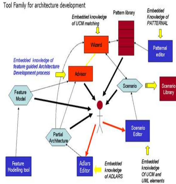
Figure 9. Overview of the QUB/ECIT tools set for feature guided architecture development which is explained further in the text.
