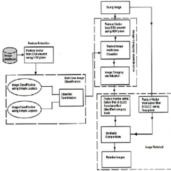
Figure 1. Proposed Algorithm based on Semantic categorization
