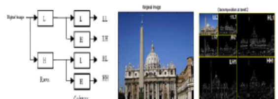
Figure 2. Wavelet Decomposition of 2D-image signal
