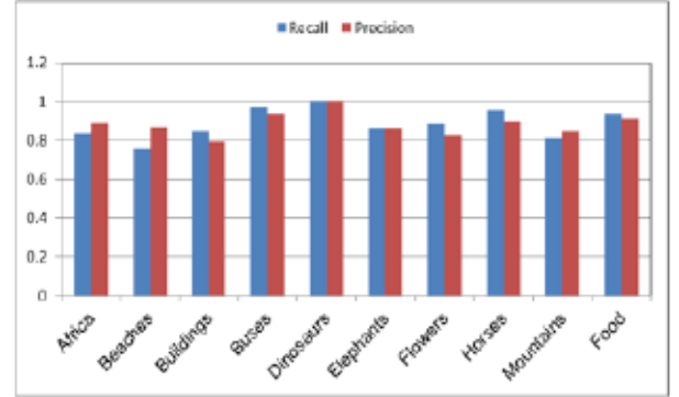
Figure 3. Classification accuracy of the combined classifier
